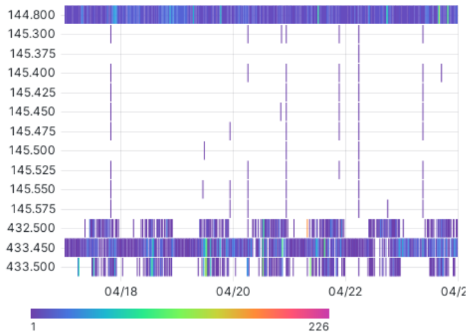
Squelch Opens
