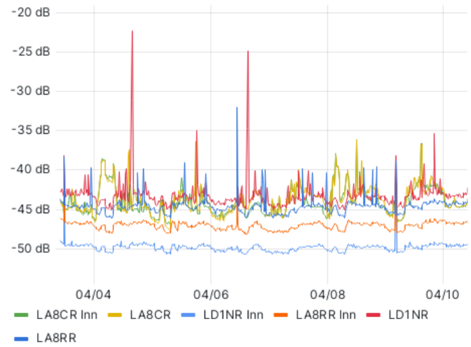
Noise Levels
