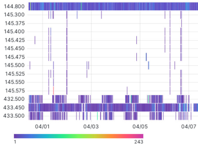
Squelch Opens
