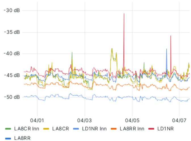
Noise Levels
